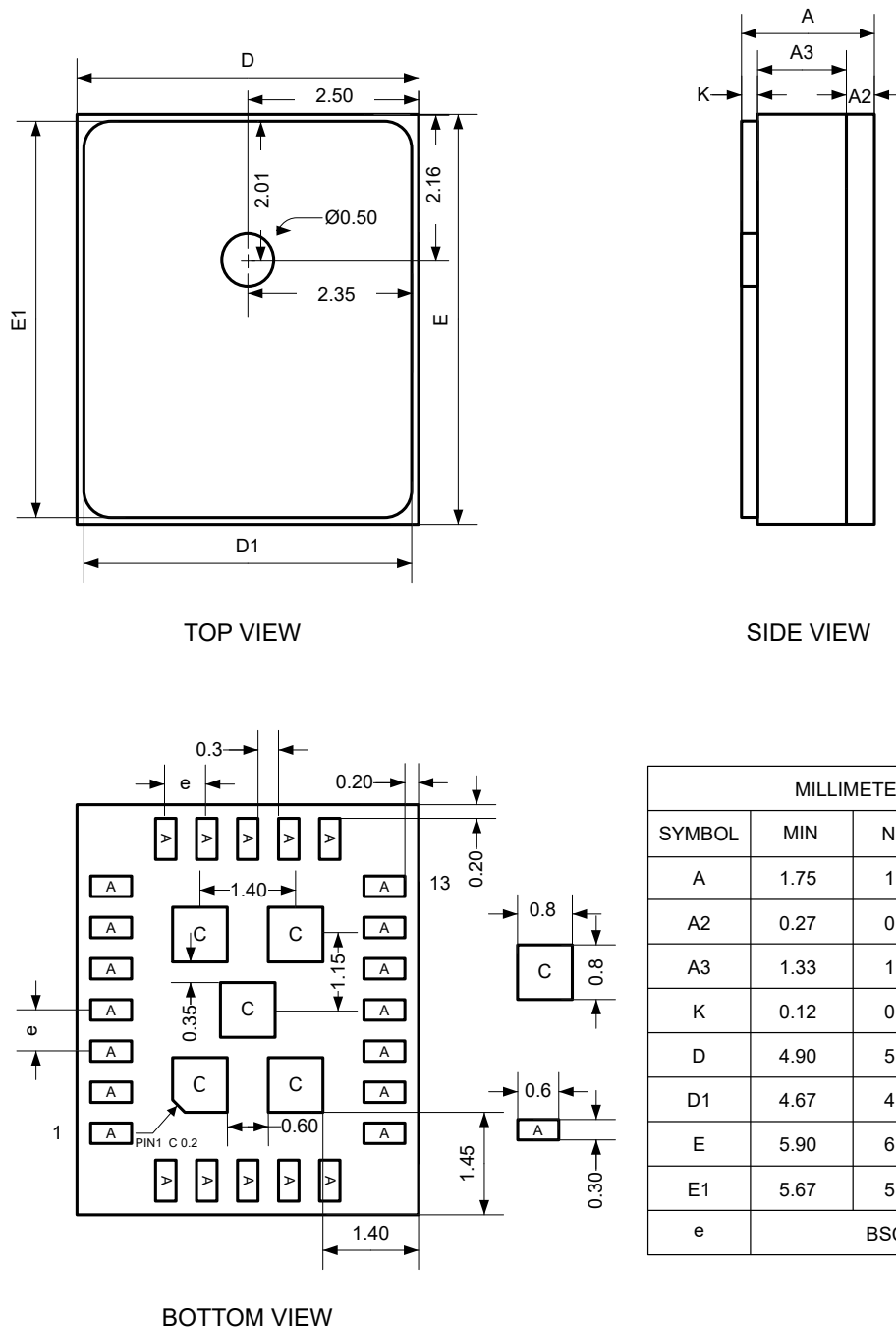
Figure 7-1 Package Outline
