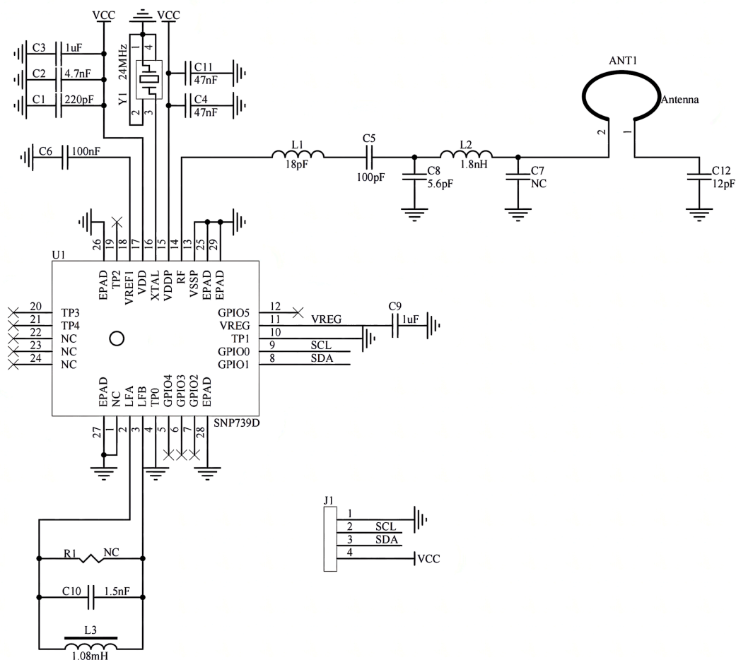
Figure 6-1 Application Circuit
