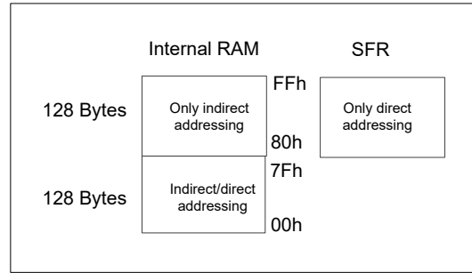
Figure 5-5 RAM/SFR map
