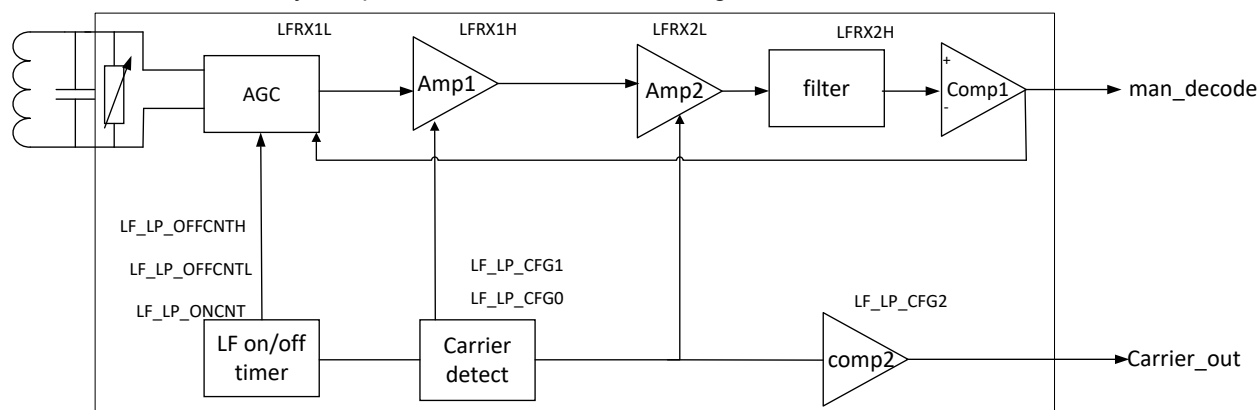
Figure 5-10 AFE
